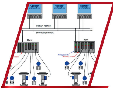
Distributed Control System
